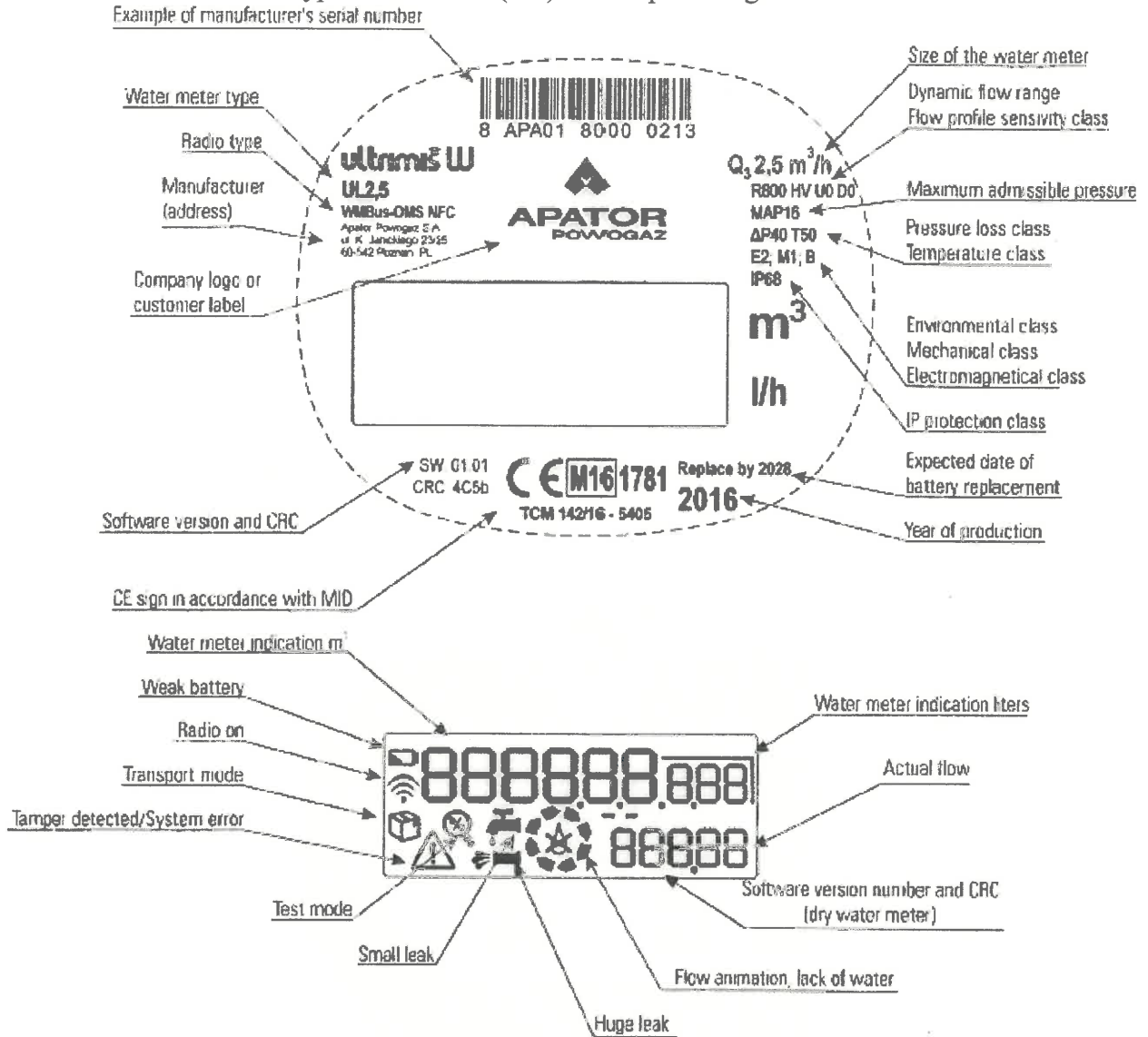
Figure 1: The water meter type ULTRIMIS (UL) – example of register:
