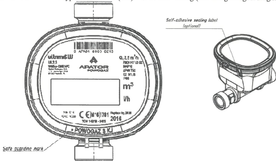
Figure 2: The water meter type ULTRIMIS (UL) – view and sealing (including safeguarding mark):
