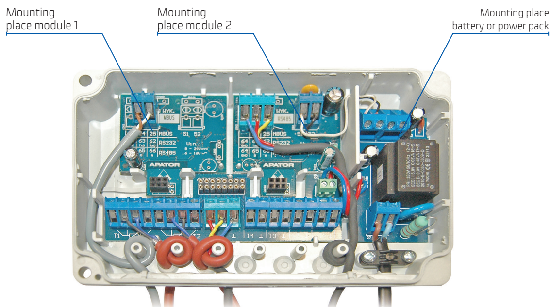
View of the base with connecting binding, with installed communication modules and plug-in power supply as well as the way of leading the cables in IP54 version.
