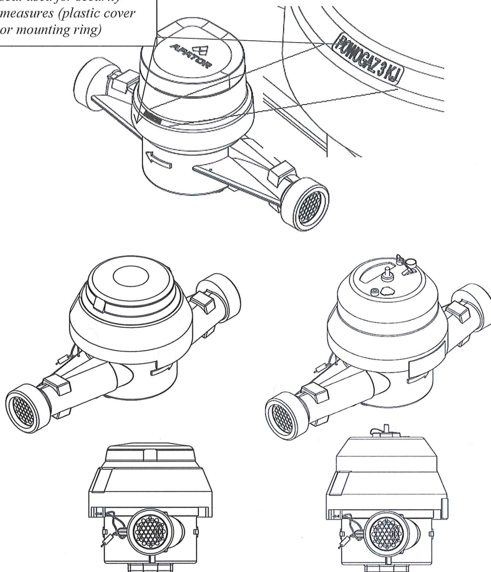
Picture No.4 Emplacement of the seal used for security measures in versions without adjusting channels with wire and round
