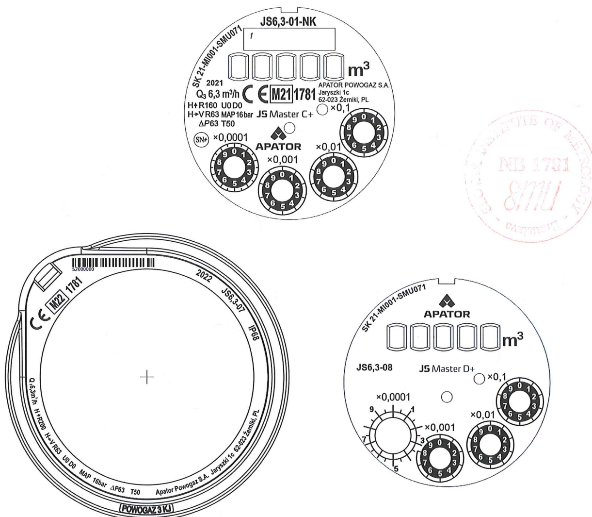
Picture No.3 Examples of the dial marking
